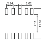
Dual Row Recommended PCB Layout (PCB TOLERANCE ±0.05)
